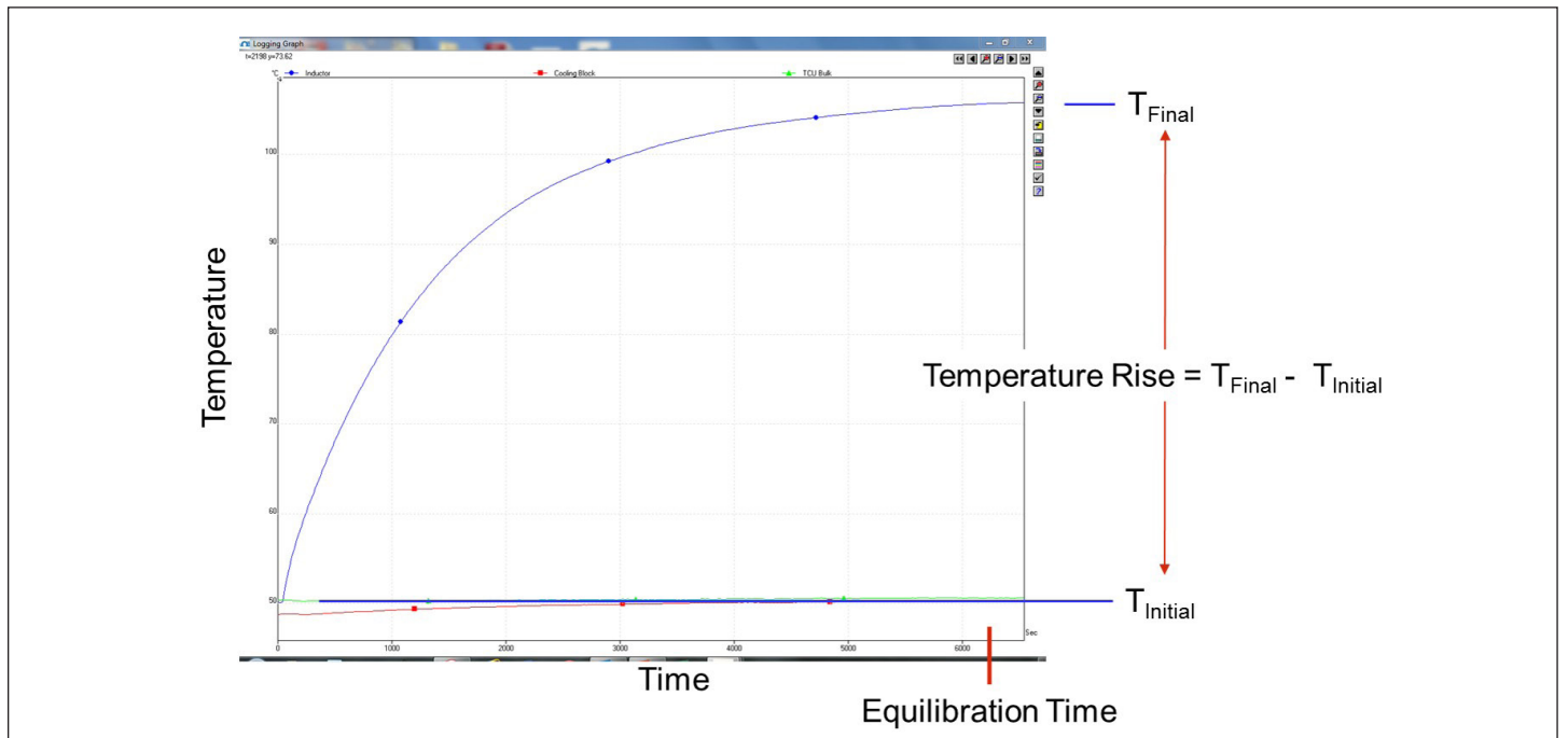
Figure 5: Temperature profile for a typical SC-400 potted inductor test, showing definitions of temperature rise and equilibration time. The blue line is the inductor, and the nearly-horizontal red line is the cooling plate.
